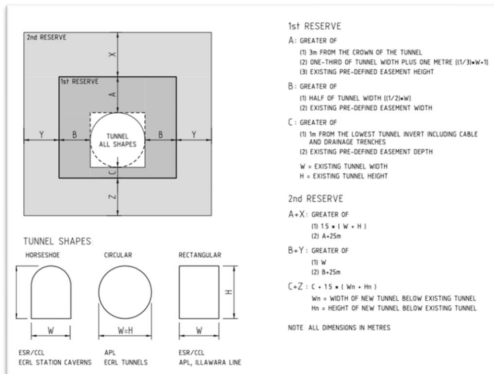
Figure 3-1 Extract from Development Near Rail Tunnels Section 5.1 (TfNSW, 2018)
